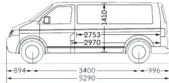
Lang "L"
